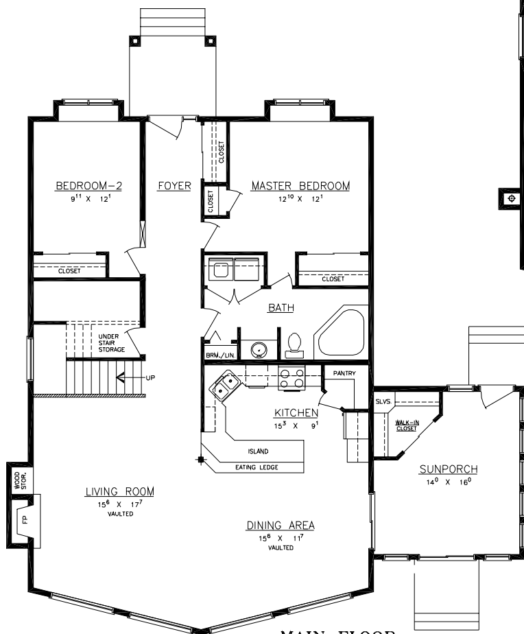
MAIN FLOOR
